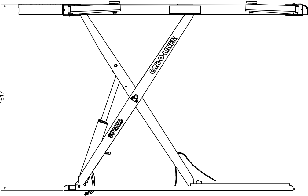
Bench and lift in upper position
