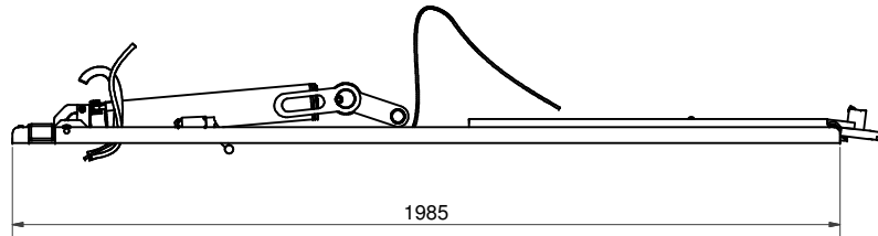
Lift platform to show cable and hydraulic output and bolting positions
